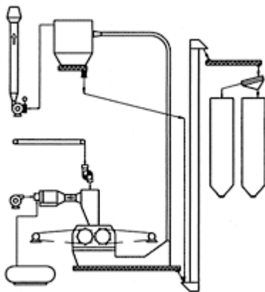
Grinding plant with BIROTOR hammer mill and dynamic separator
