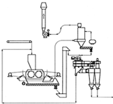
Combined grinding and drying plant with Birotor hammer mill
